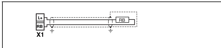
Figure 3.9 Braking resistor connection
