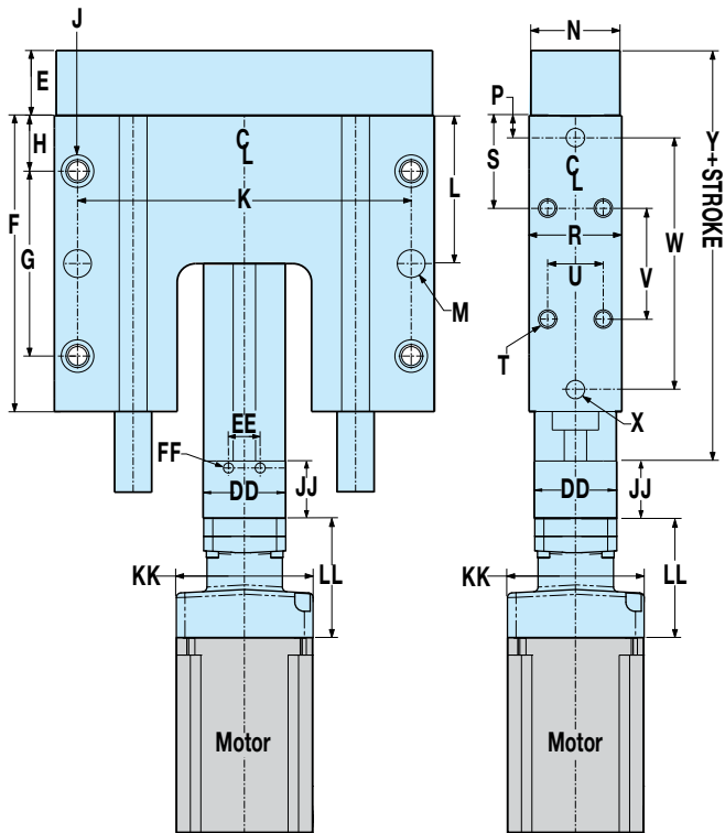
LMI Motor Mount
